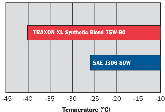
TRAXON (Low Temperature Performance) SAE J306 (°C) @ 150,000 cP
