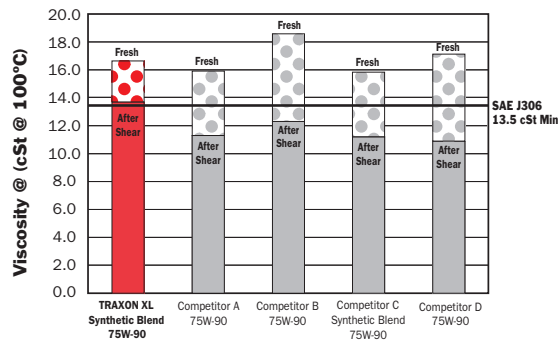
75W-90 SAE J306, Gear Oils / Fresh and after KRL Viscosities @ 100°C
